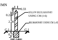
CROSS SECTION OF COMPOUND WALL.
