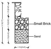
SECTION OF RAIN WATER COLLECTION PITS (INTS)
