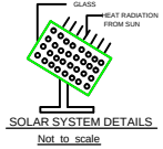
SOLAR SYSTEM DETAILS Not to scale
