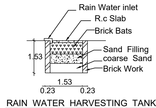
RAIN WATER HARVESTING TANK
