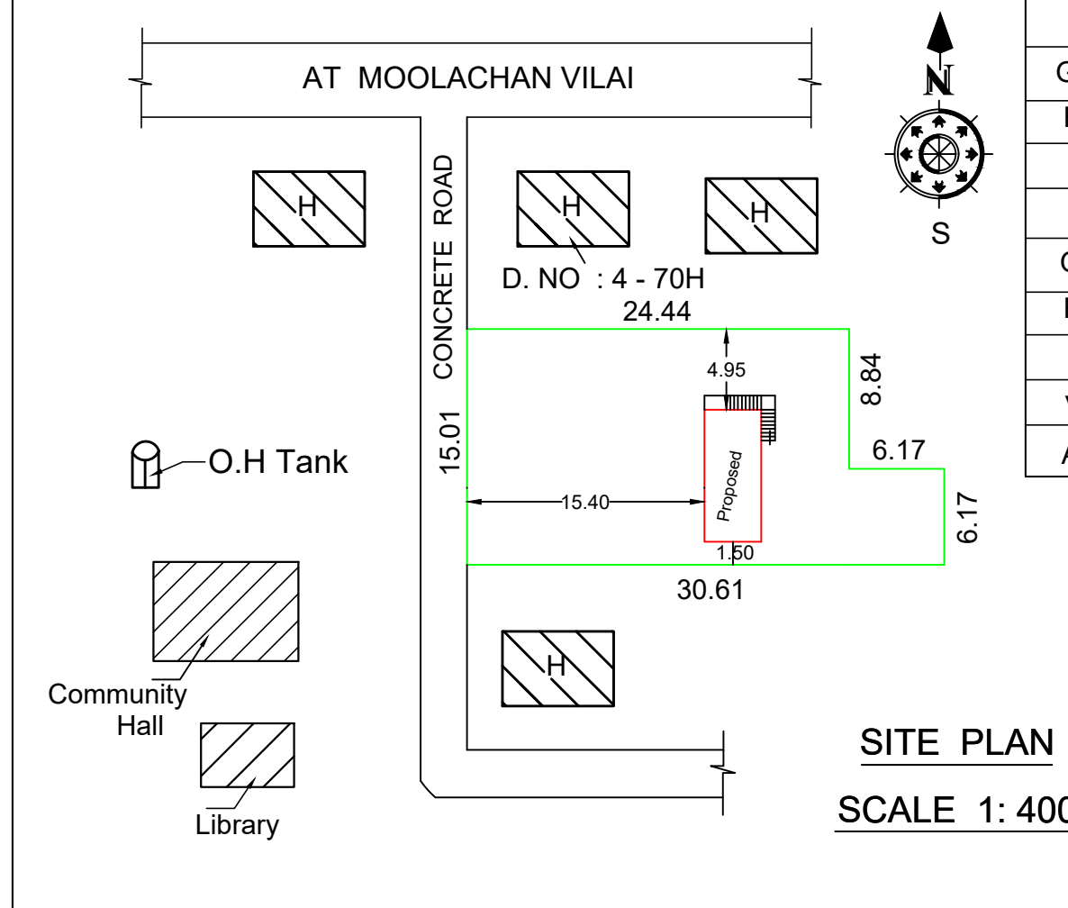
RAIN WATER HARVESTING TANK
