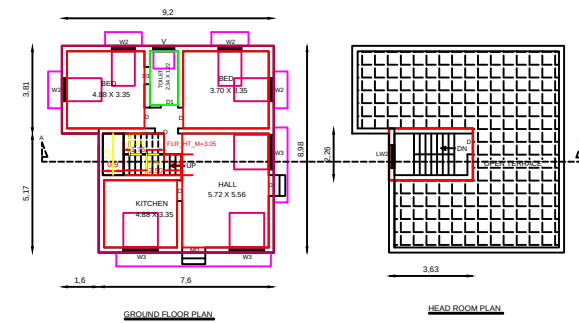
HEAD ROOM PLAN
