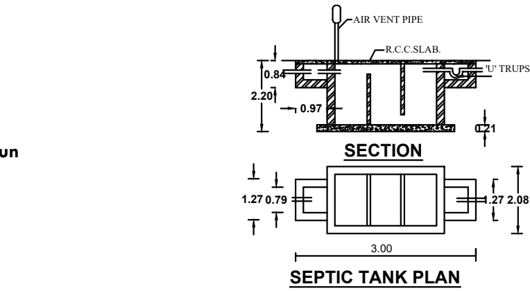
SEPTIC TANK PLAN
