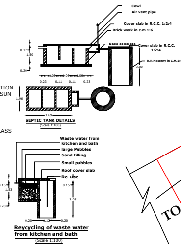
Recycling of waste water from kitchen and bath
