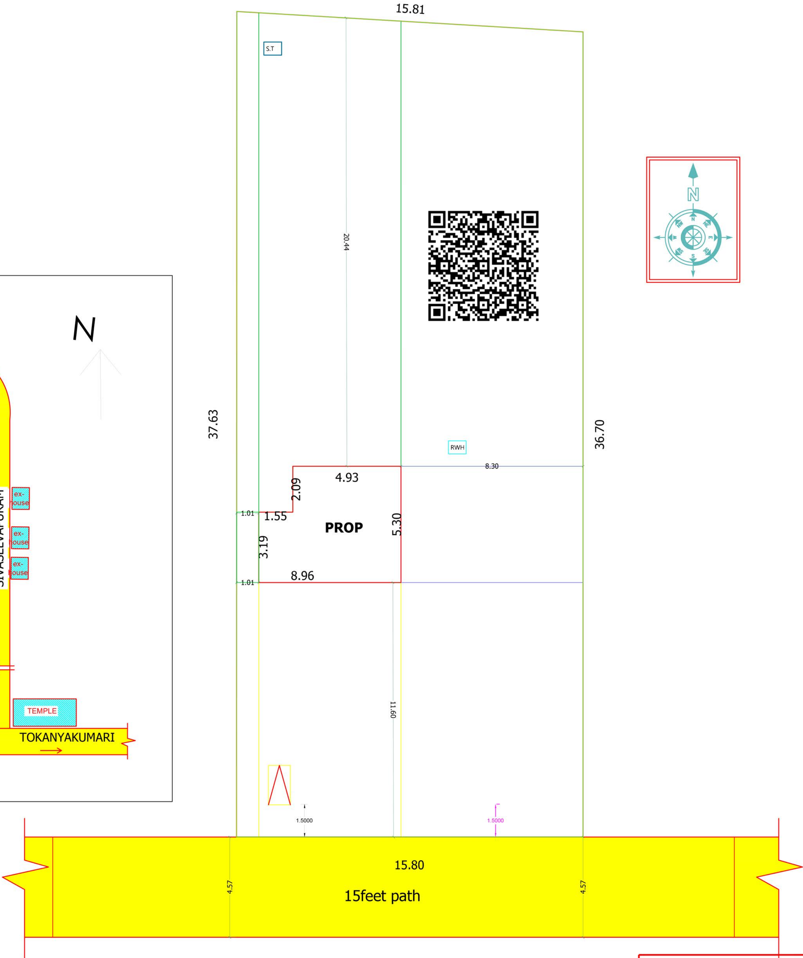
SITE PLAN
