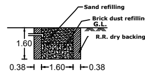
DETAILS OF RAIN WATER HARVESTING
