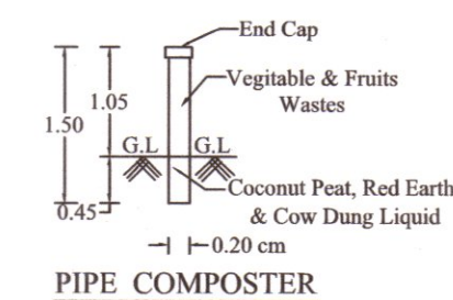
PIPE COMPOSTER
