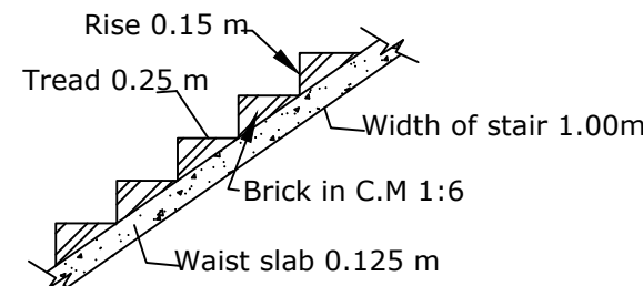
STAIR DETAILS
