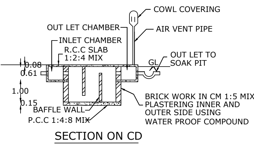
SECTION ON CD
