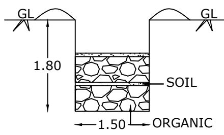
COMPOST PIT
