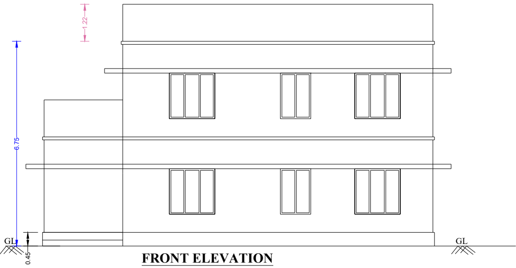
FRONT ELEVATION
