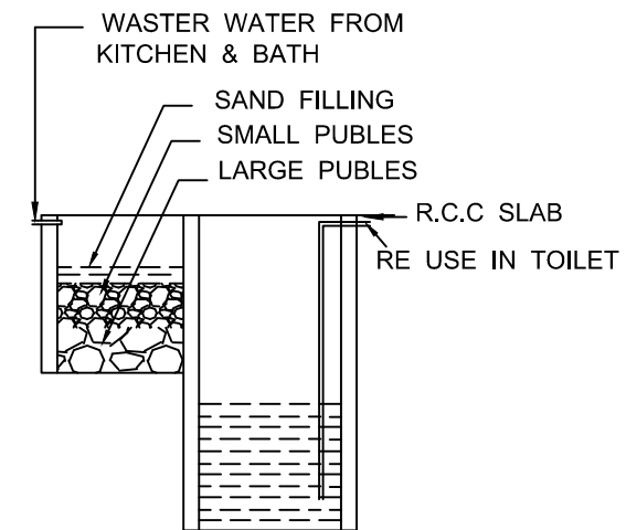
RECYCLING OF WASTE WATER KITCHEN & BATH ROOM
