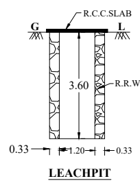
LEACH PIT
