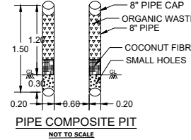
PIPE COMPOSITE PIT NOT TO SCALE
