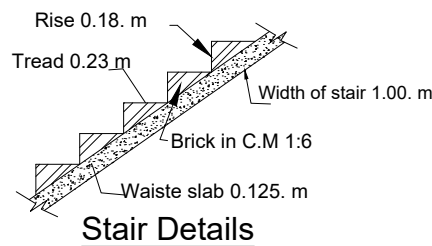
Stair Details
