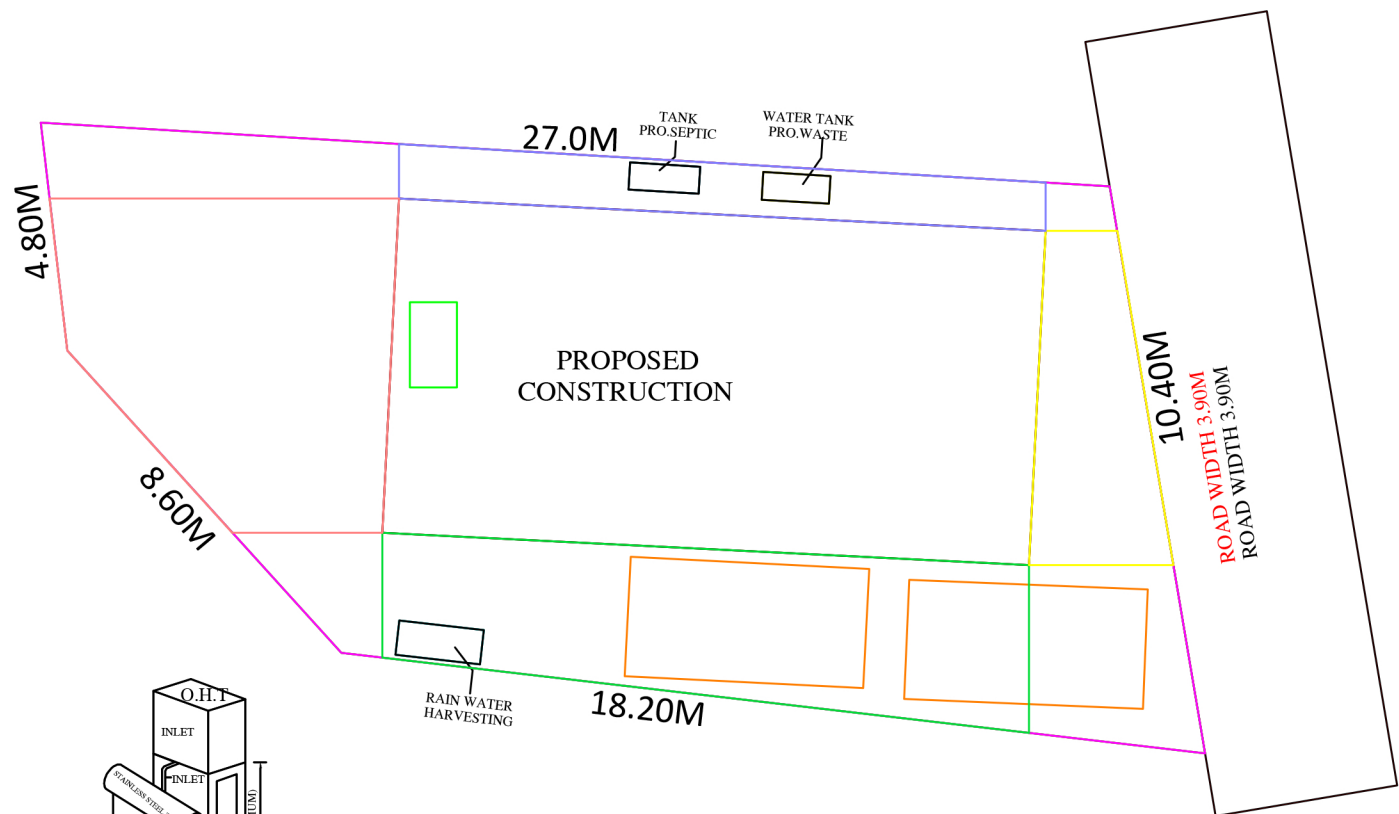
SITE PLAN
