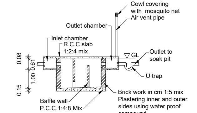
SECTION UV
