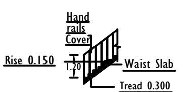
STAIRCASE DETAILS
