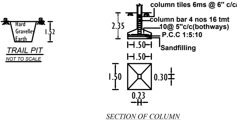
SECTION OF COLUMN
