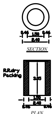
RAIN WATER HARVESTING ARRANGEMENT
