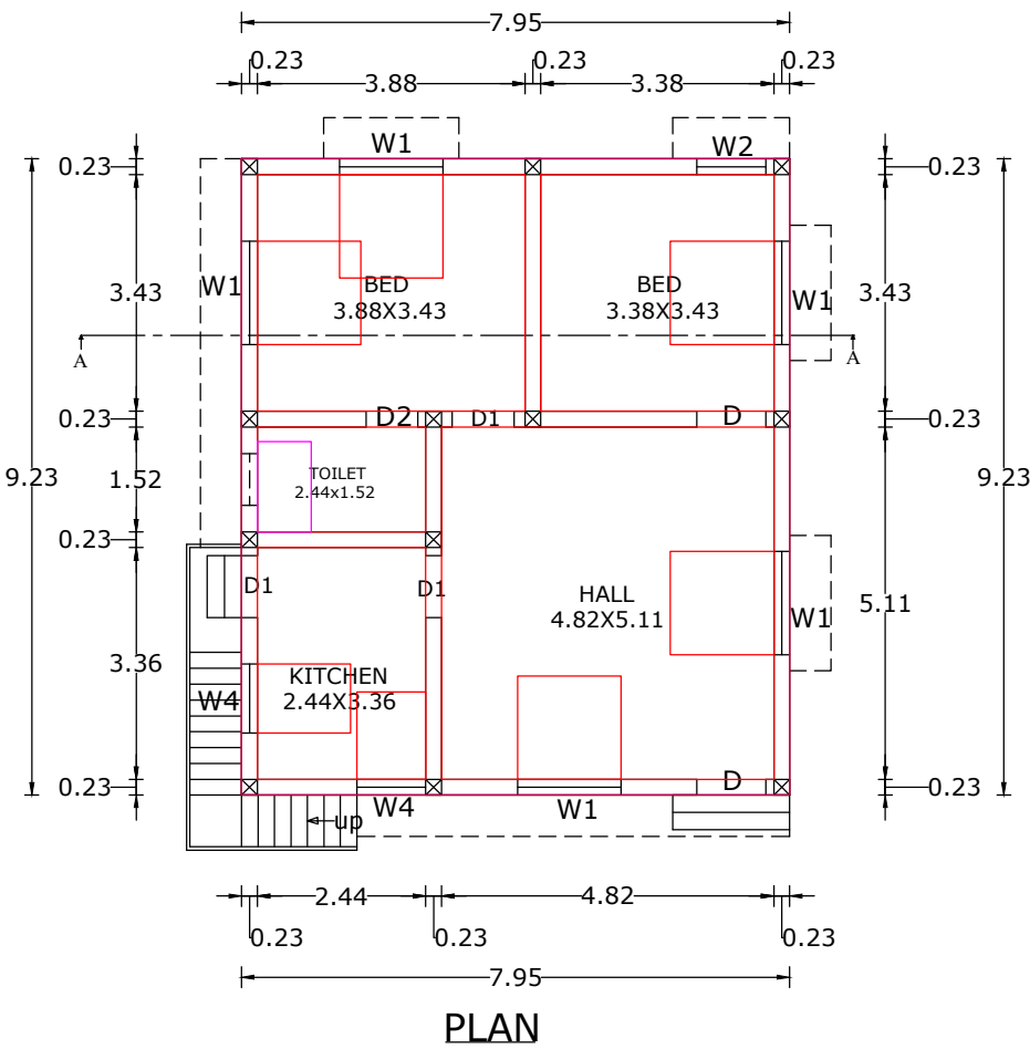
PLAN
