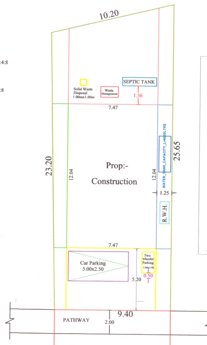
SITE PLAN
