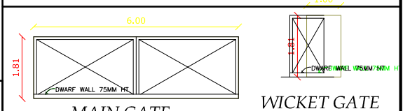
MAIN GATE
