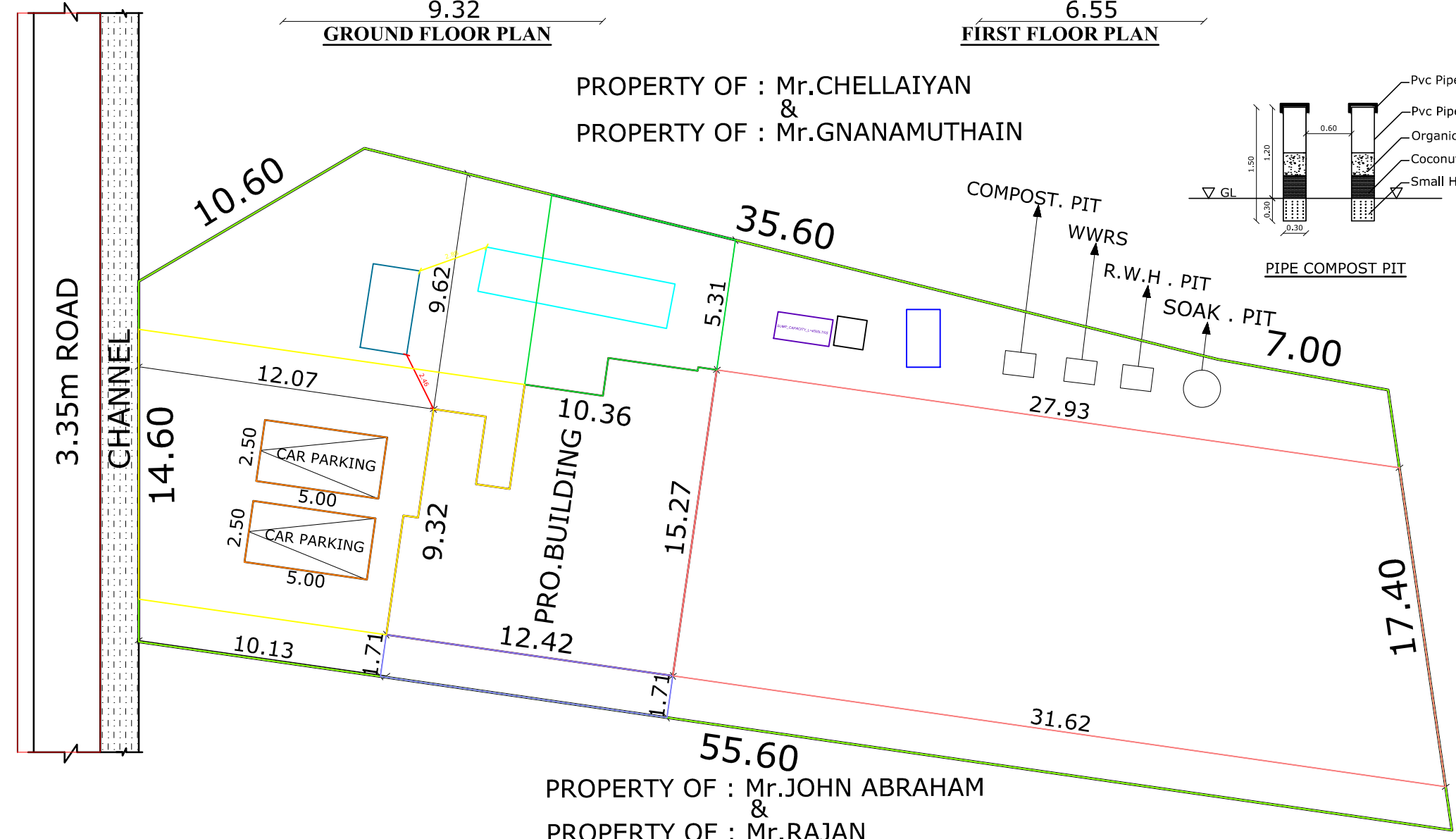
SITE PLAN
