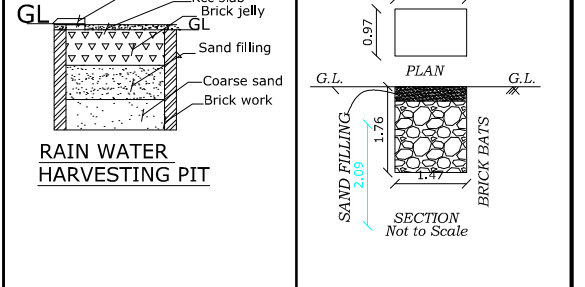
DETAILED PLAN OF RAINWATER PERCOLATION PEBBLE BED
