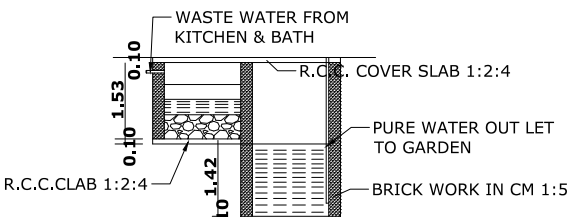
RECYCLING OF WASTE WATER SYSTEM
