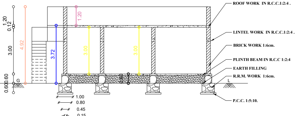
SECTION ON-AB
