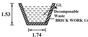
WASTE PIT
