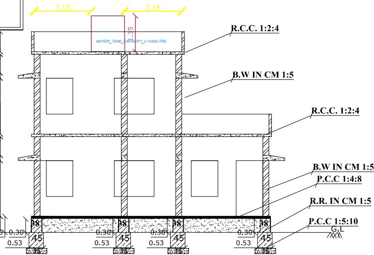
CROSS SECTION ON 'AB'
