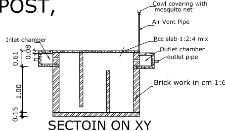
SECTION ON XY
