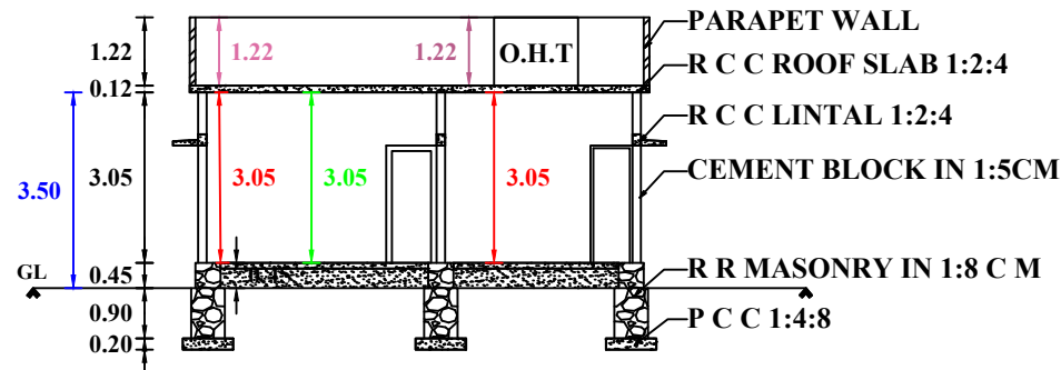
SECTION ON X-Y
