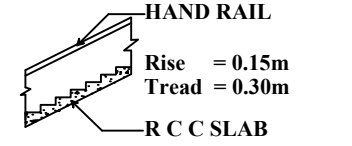
DETAILS OF STAIR CASE
