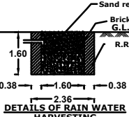
DETAILS OF RAIN WATER HARVESTING Dwg:1A
