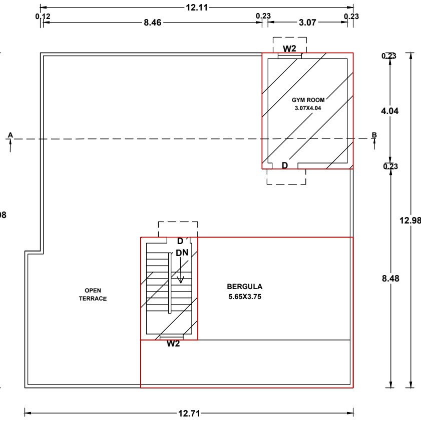
EXISTING, PROPOSED SECOND FLOOR PLAN
