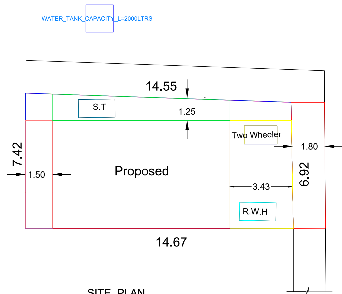
SITE PLAN
