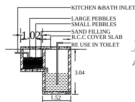
DETAILS OF RECYCLING OF WASTE
