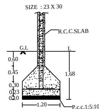
DETAILS OF R.C.C COLUMN
