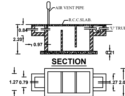
SEPTIC TANK PLAN
