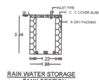
RAIN WATER STORAGE TANK SECTION
