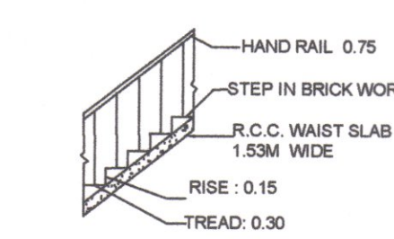
STAIR CASE SECTION
