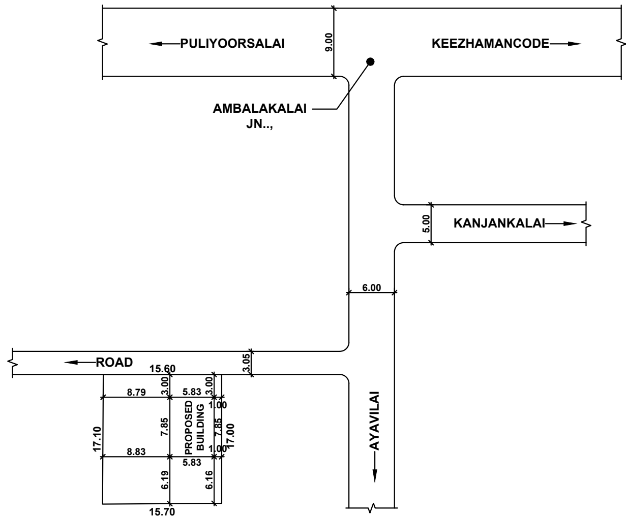
KEY PLAN SCALE:1:400.
