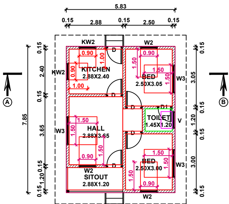
PLAN
