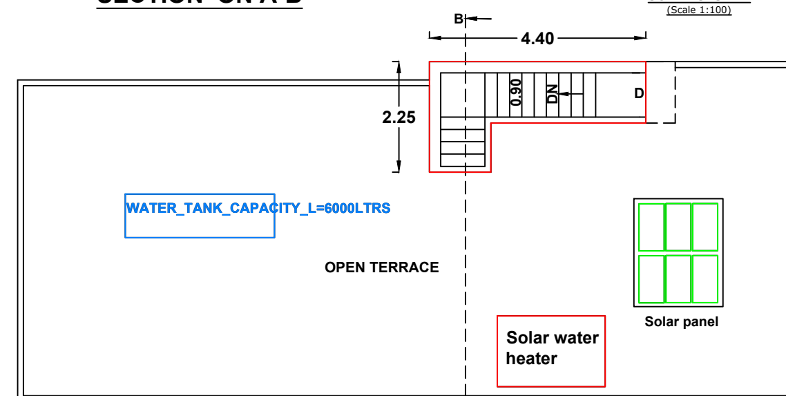
HEAD ROOM PLAN
