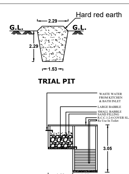
RECYCLING OF WASTE WATER FROM KITCHEN & BATHROOM
