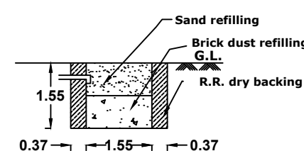
DETAILS OF RAIN WATER HARVESTING Dwg:1A
