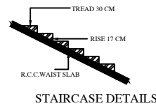
STAIRCASE DETAILS
