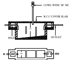
SEPTIC TANK DETAILS
