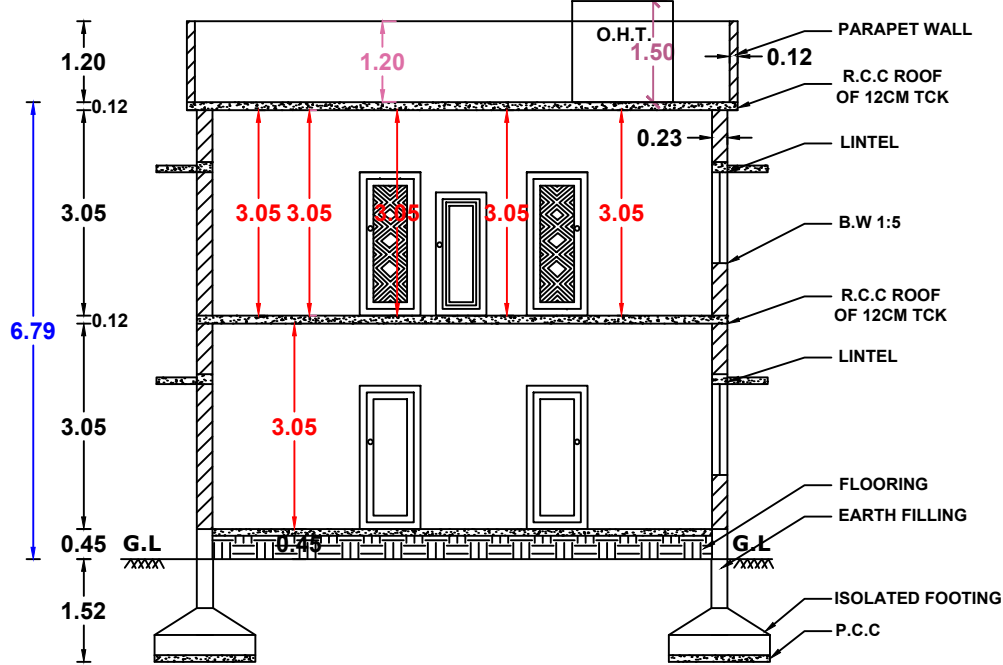
SECTION-AA & BB
