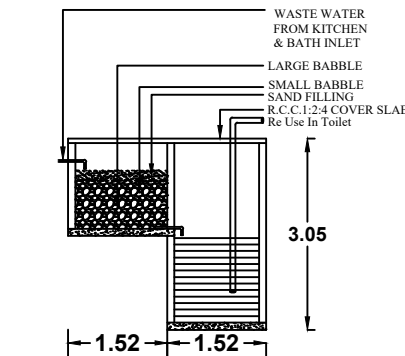
RECYCLING OF WASTE WATER FROM KITCHEN & BATHROOM
