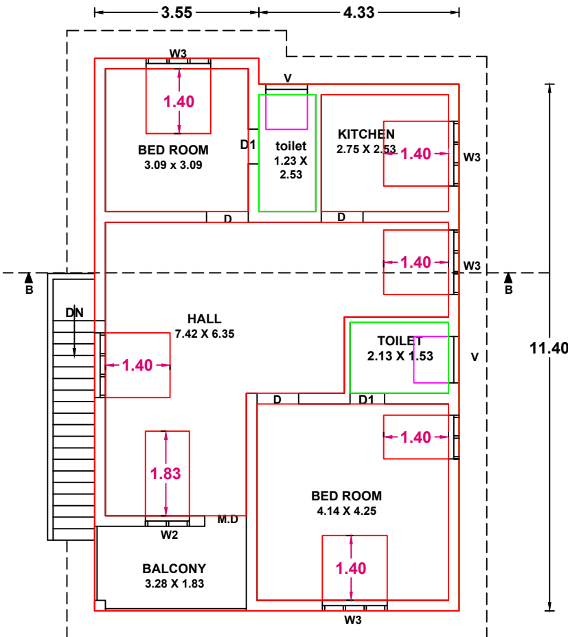
F. FLOOR PLAN
