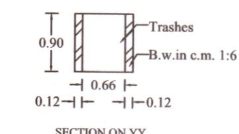
SECTION ON YY'
