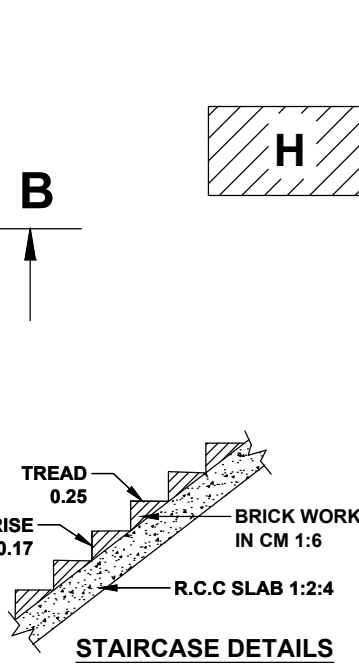
STAIRCASE DETAILS
