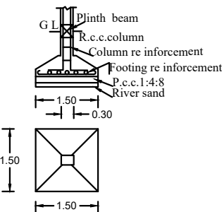
Column detail
