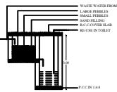
RECYCLING OF WASTE WATER FROM BATH
