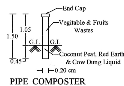
PIPE COMPOSTER
