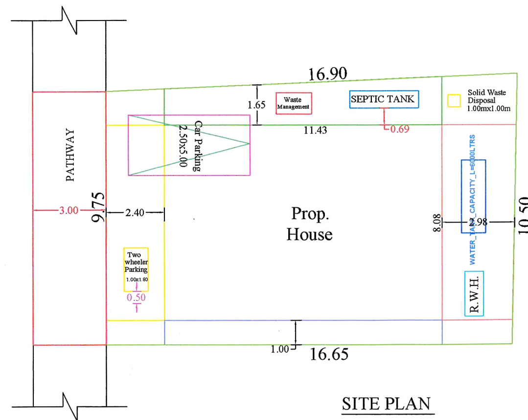
RAIN WATER HARVEST WELL RWH CAPACITY L=6642LTRS
