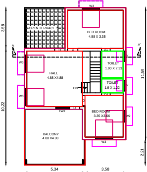
FIRST FLOOR PLAN (BLOCK-I)
