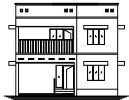
ELEVATION (BLOCK-I)
