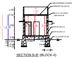
SECTION B-B' (BLOCK-II)
