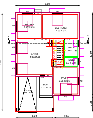
GROUND FLOOR PLAN (BLOCK-I)
