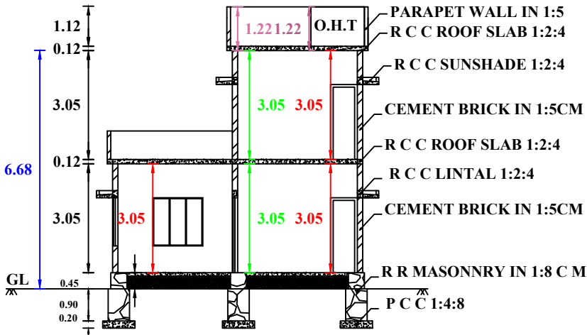
SECTION 'X-Y'
