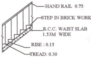
STAIR CASE SECTION
