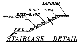
STAIRCASE DETAIL
