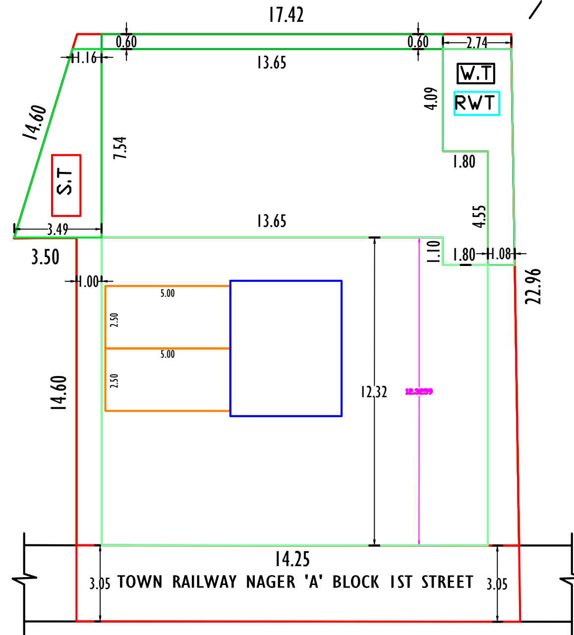
SITE PLAN
