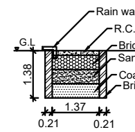
RAIN WATER HARVESTING PIT
