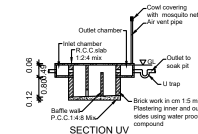
SECTION UV
