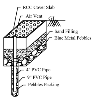
Percolation Bore Pit
