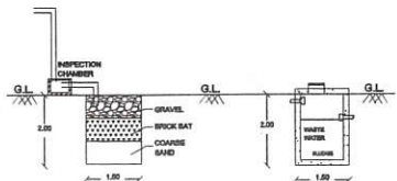
RAIN WATER HARVESTOR
