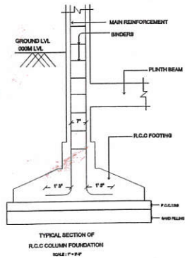
TYPICAL SECTION OF R.C.C COLUMN FOUNDATION
