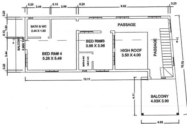
Prop. FIRST FLOOR PLAN
