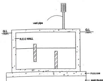
SECTION ON BB
