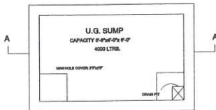
SUMP PLAN
