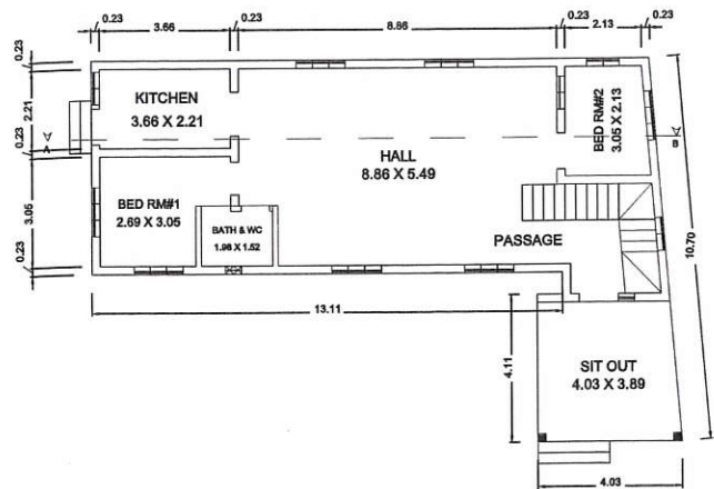
Prop. GROUND FLOOR PLAN
