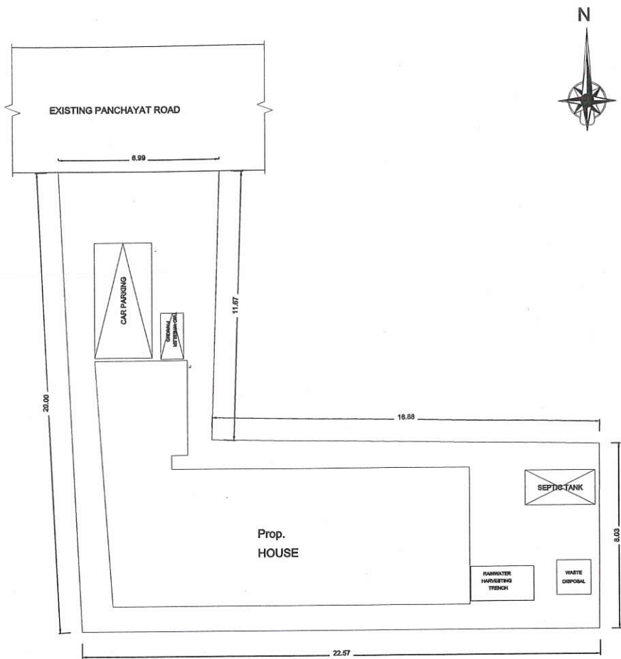
SITE PLAN
