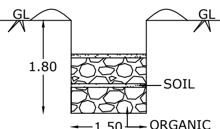
COMPOST PIT
