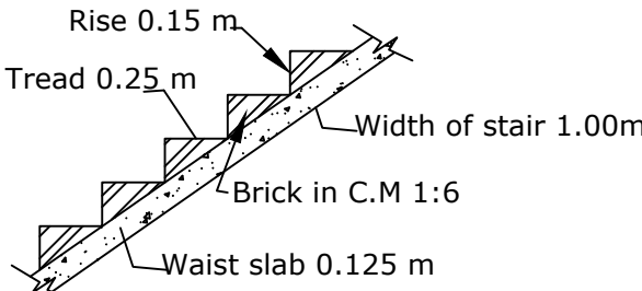
STAIR DETAILS
