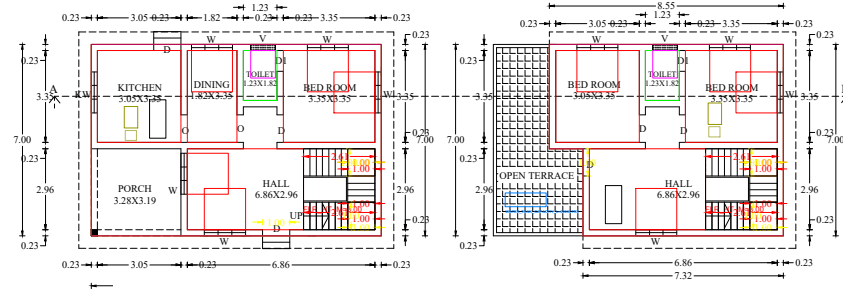
RST FLOOR (scale - 1:100)
