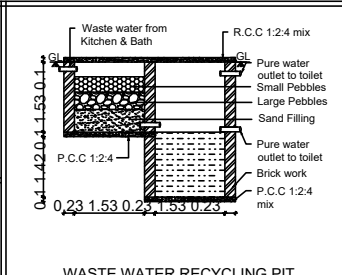
WASTE WATER RECYCLING PIT
