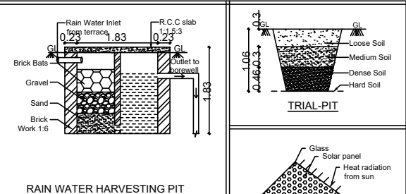
RAIN WATER HARVESTING PIT
