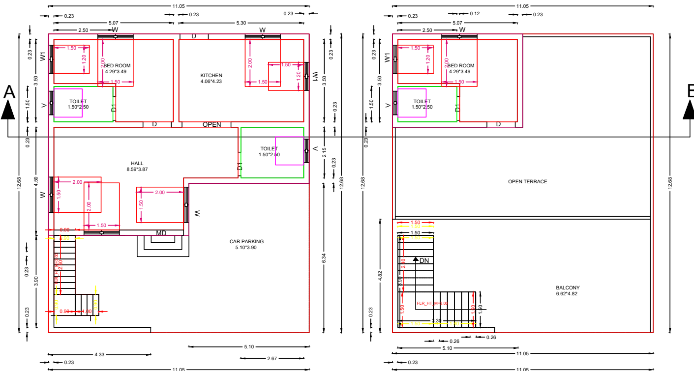
FIRST FLOOR
