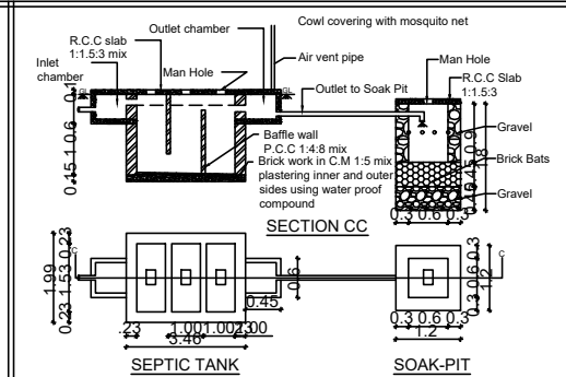
SEPTIC TANK
